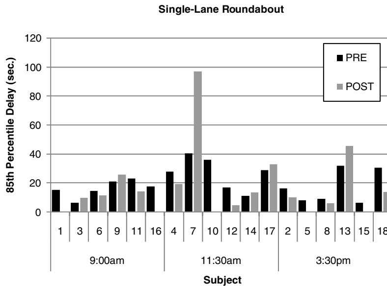
Exhibit 19. 85th percentile delay by subject – single-lane roundabout.
