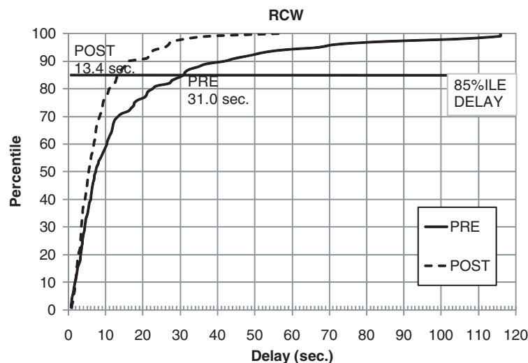
Exhibit 39. Cumulative delay distribution of pedestrian delay at RCW.
