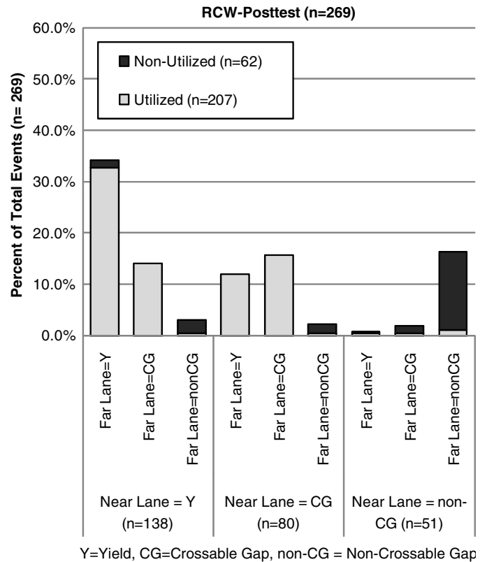
Y=Yield, CG=Crossable Gap, non-CG = Non-Crossable Gap This figure shows a bar chart of all observed pedestrian-vehicle events during the RCW posttest. The graph shows a total of nine event categories, representing all combinations of event outcomes yield, crossable gap, and non-crossable gap for two conflicting lanes (near lane and far lane).
