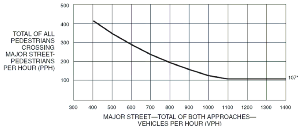
Figure 3. Warrant 4, pedestrian four-hour volume (source: FHWA 2009).
